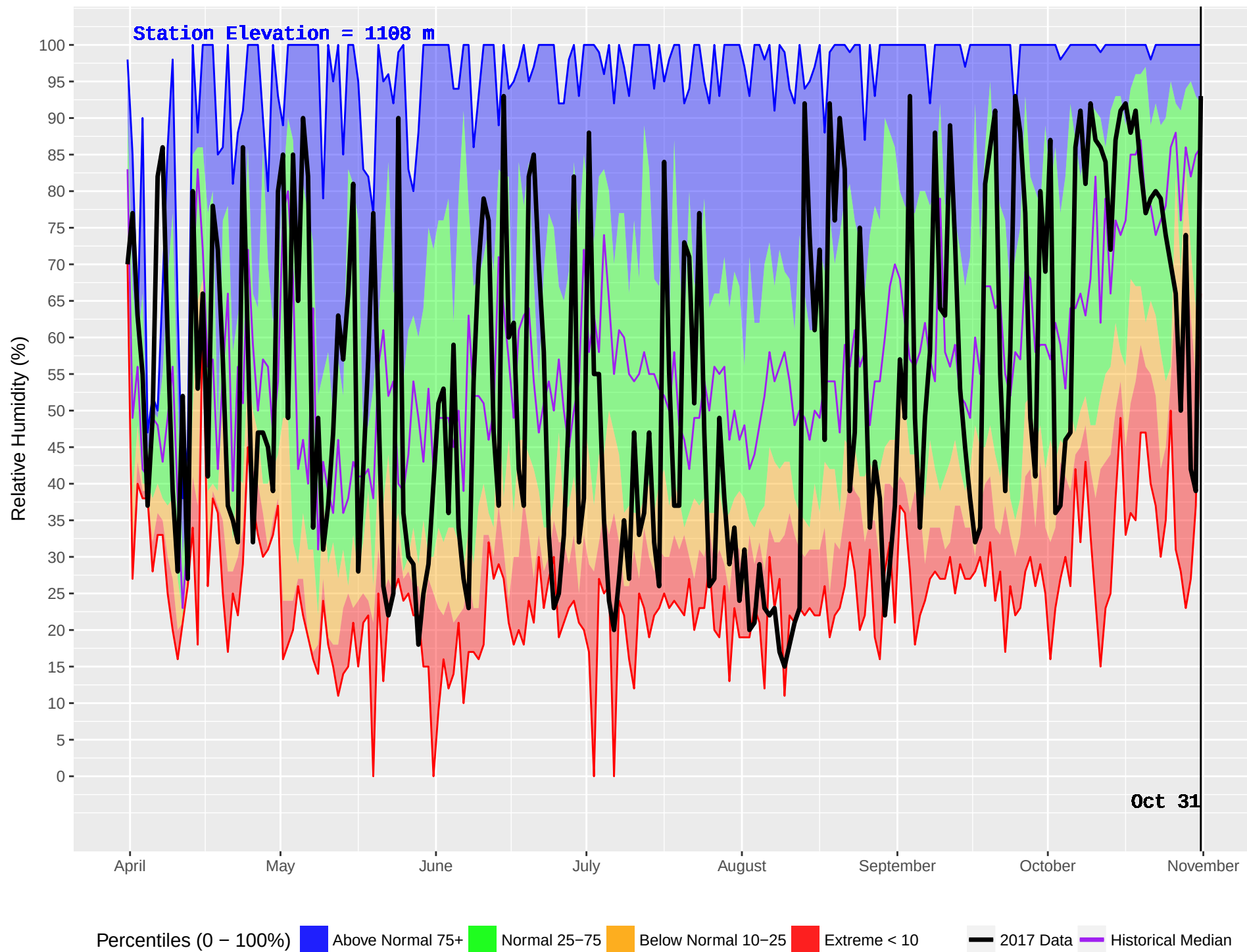
MATHEW (263) : Historical (1987–2016) and Current (2017) Noon Relative Humidity
