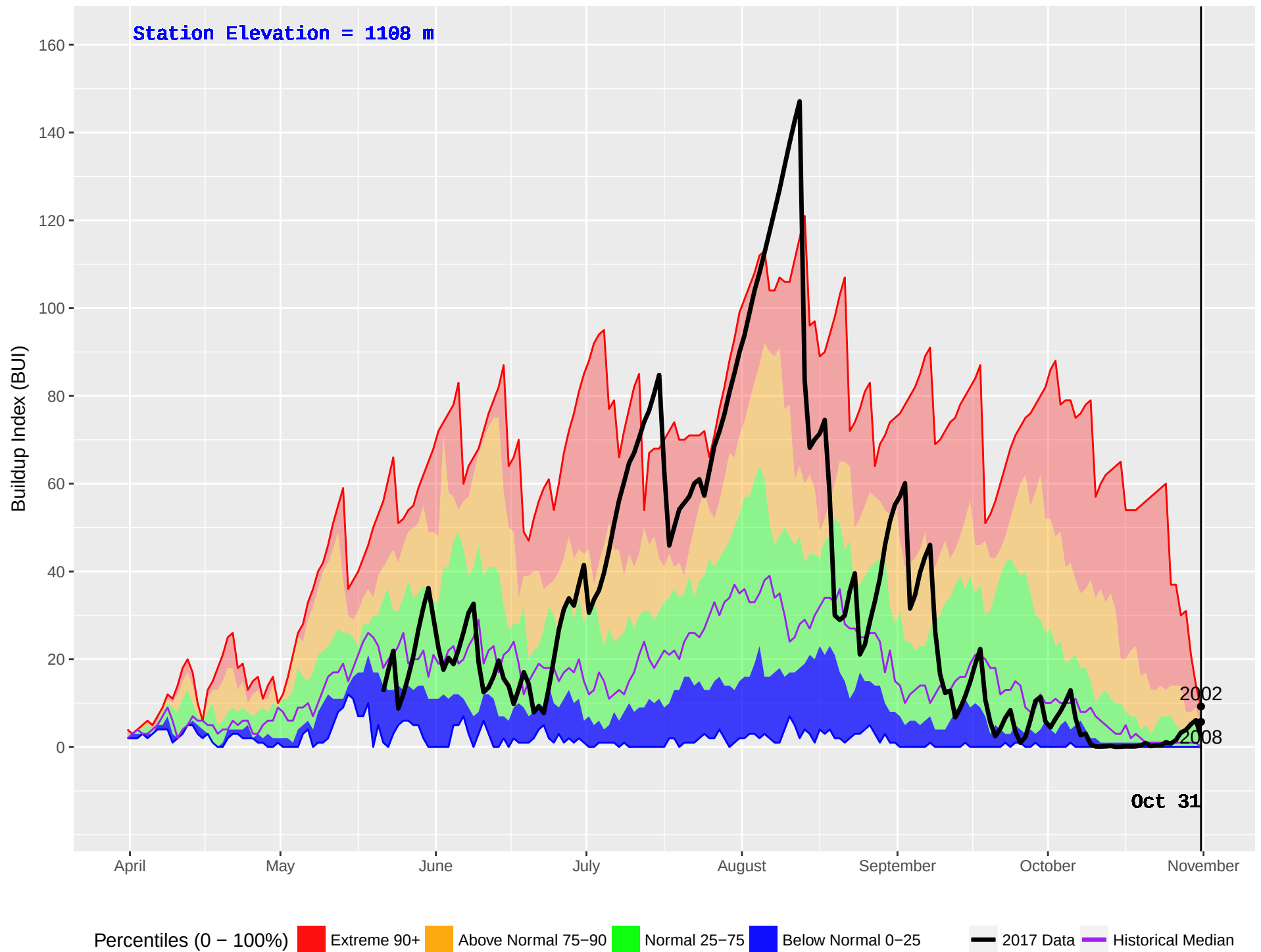
MATHEW (263) : Historical (1987–2016) and Current (2017) Noon Buildup Index (BUI)
